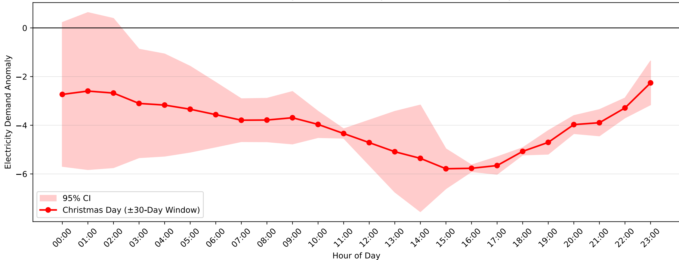
Bass Hill Demand Anomaly: Christmas Day (2008–2009, \pm 30 -Day Window)
