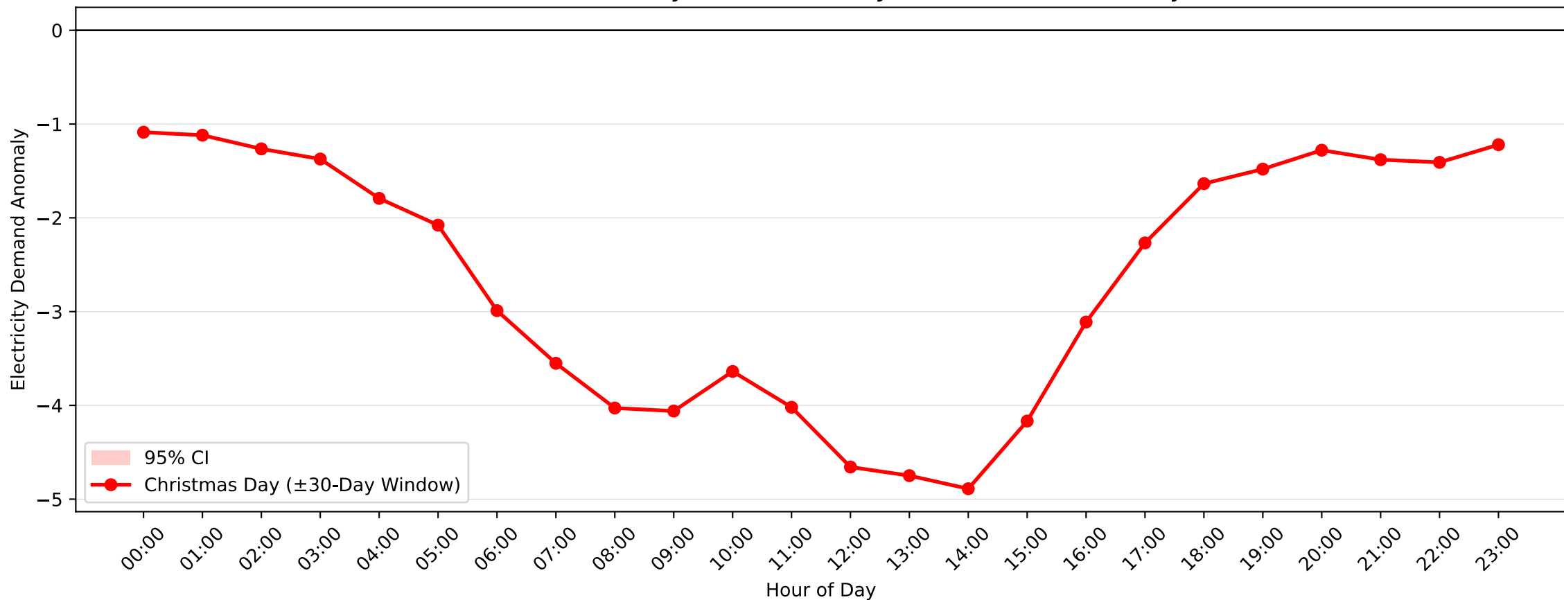
Bass Hill Demand Anomaly: Christmas Day (2004–2005, \pm 30 -Day Window)
