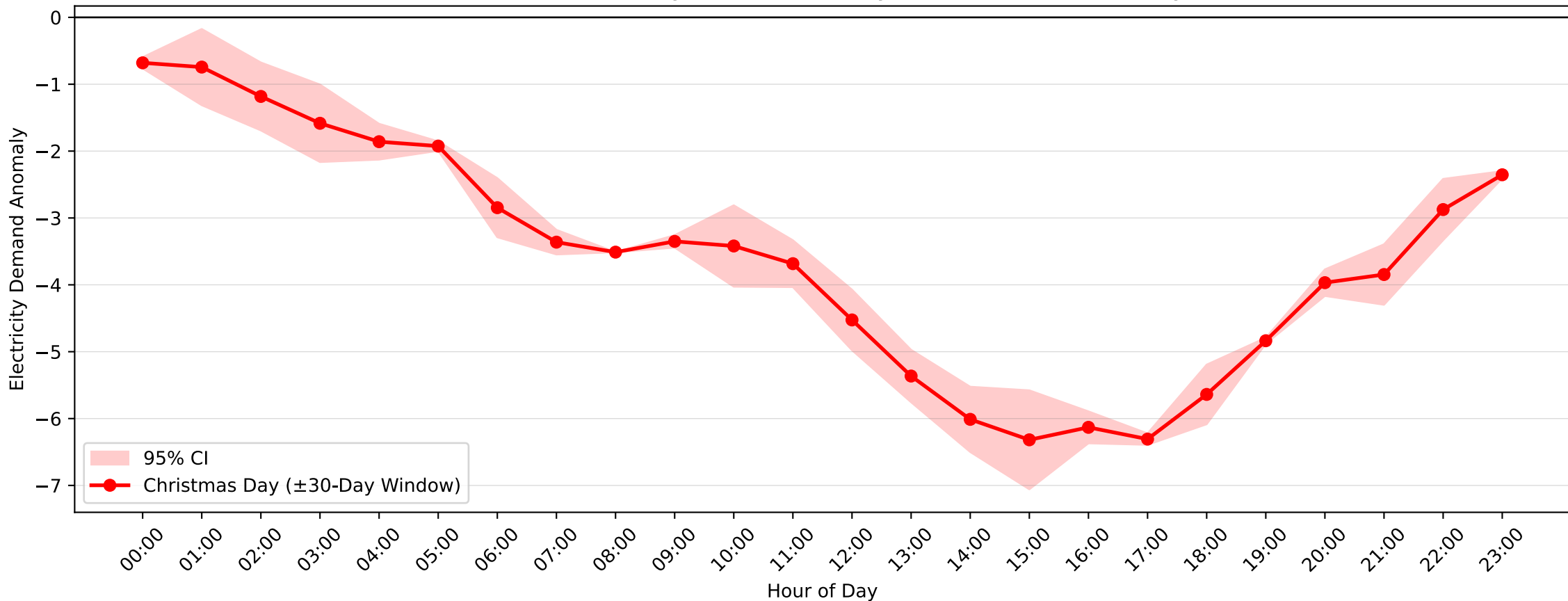
Bass Hill Demand Anomaly: Christmas Day (2006–2007, \pm 30 -Day Window)
