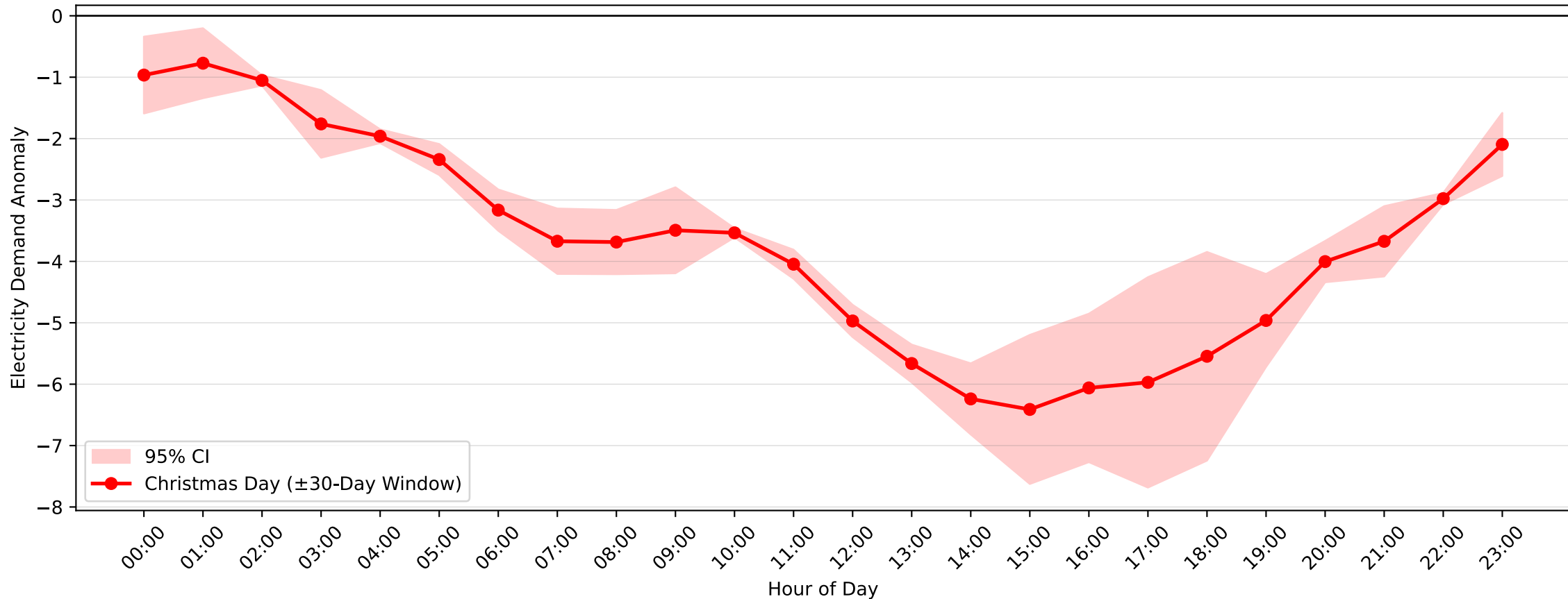
Bass Hill Demand Anomaly: Christmas Day (2007-2008, \pm 30 -Day Window)
