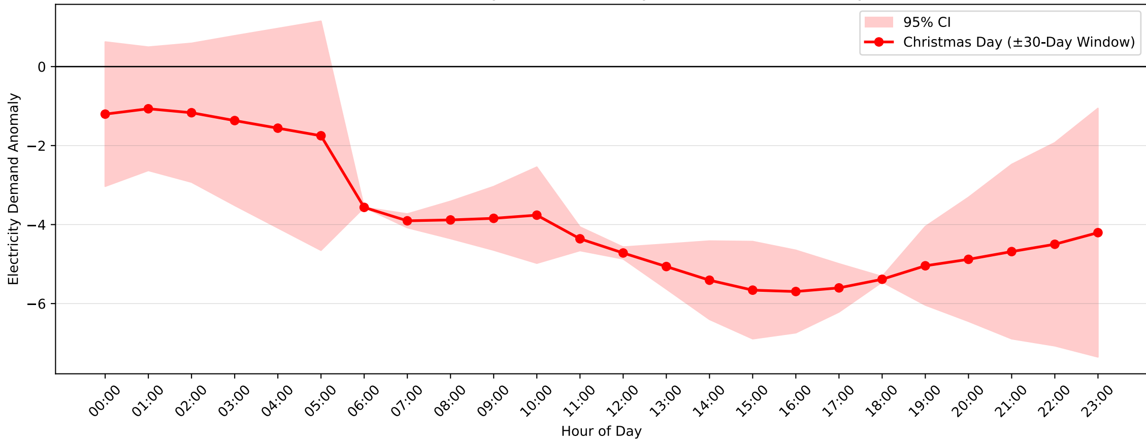
Bass Hill Demand Anomaly: Christmas Day (2014–2015, \pm 30 -Day Window)
