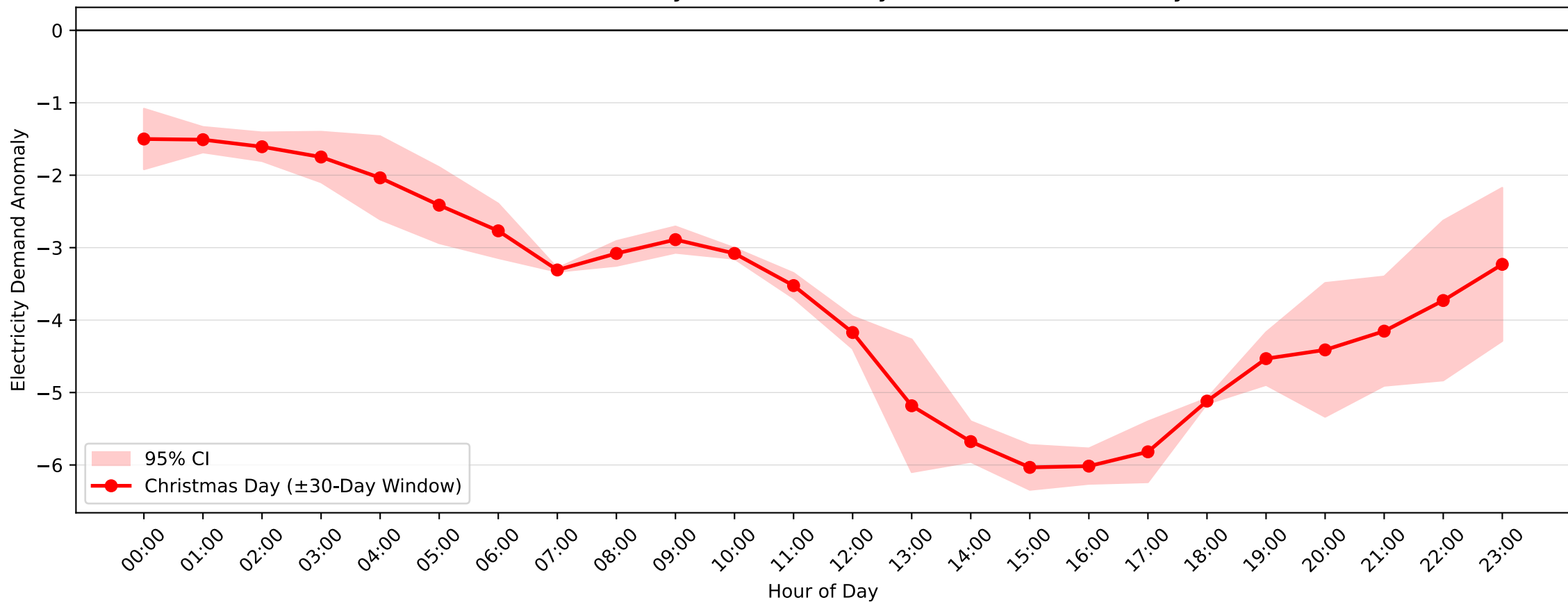
Bass Hill Demand Anomaly: Christmas Day (2012–2013, \pm 30 -Day Window)
